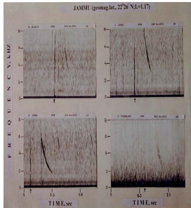
Fig. 2: Frequency –Time spectrograms of whistlers recorded at Jammu.
