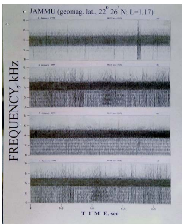
Fig. 1: Spectrograms of simultaneously observed hiss emission.
